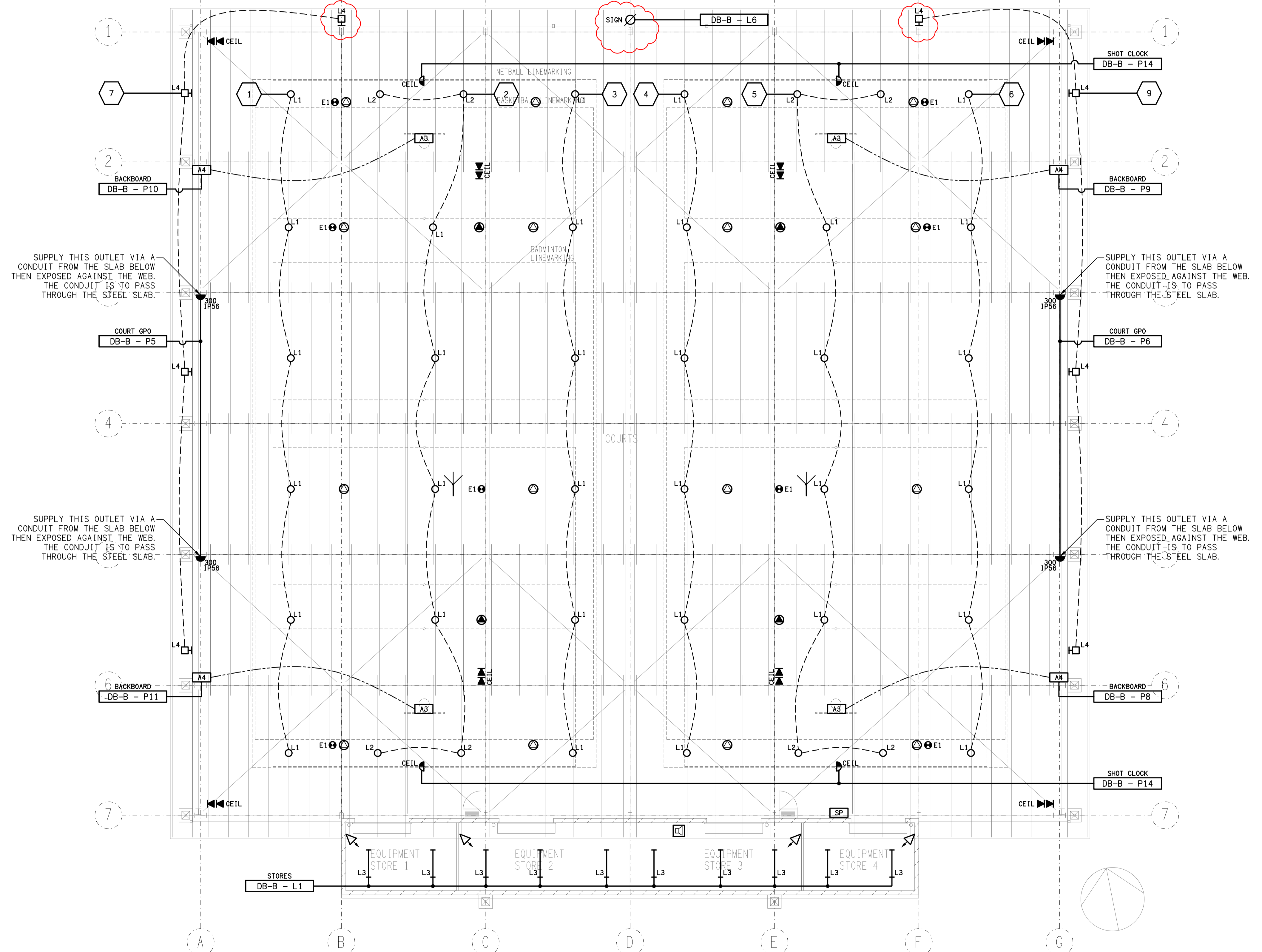
EQUIPMENT STORE ROOMS FLOOR PLAN SCALE 1:100
